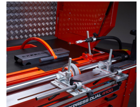
Powered clamp, reel cable drive and improved positioning scales
